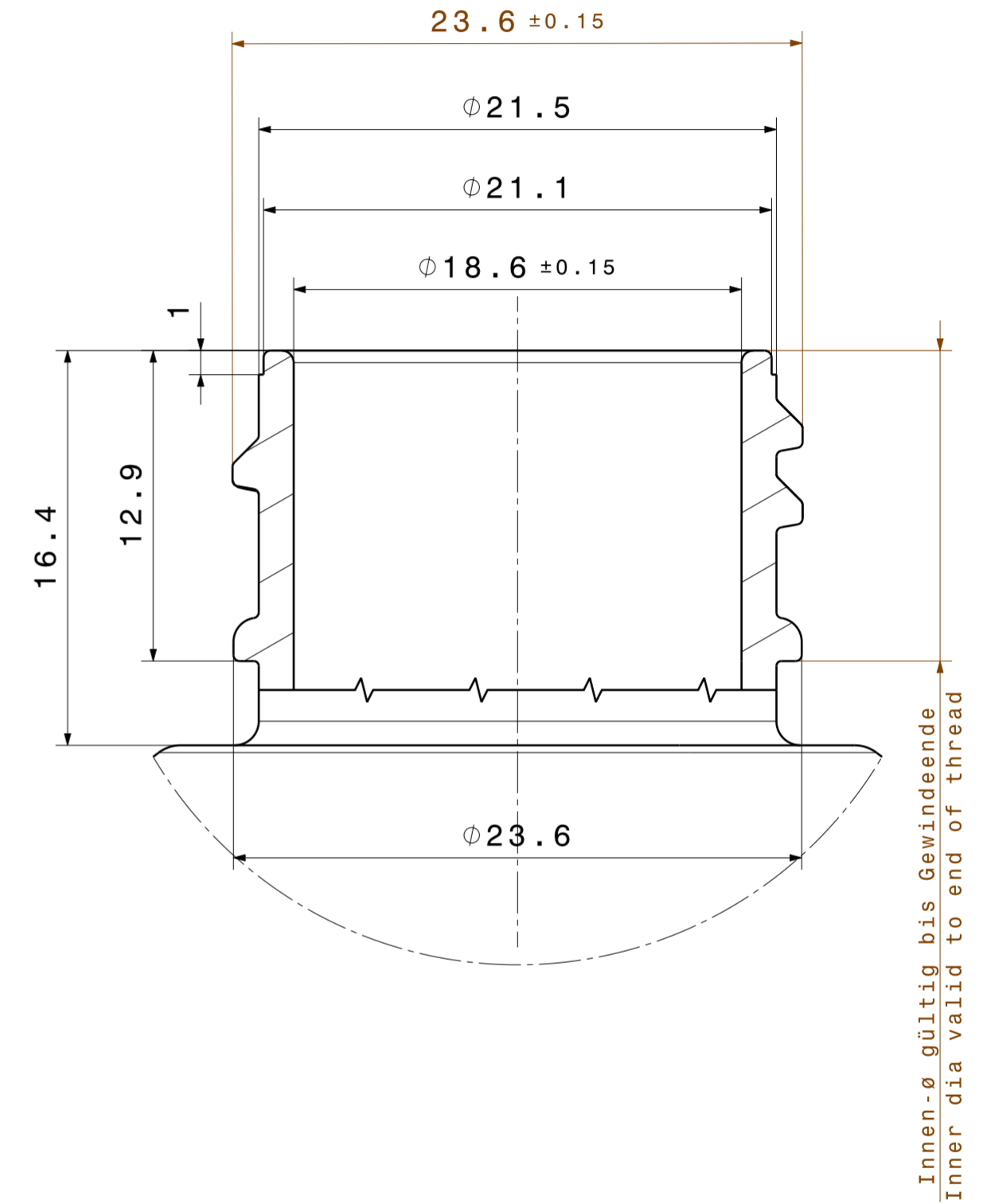
Detail A 4:1
