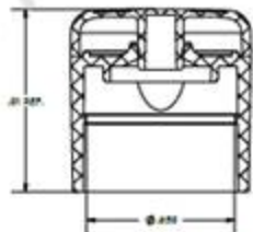
SECTION F-F SCALE 2 : 1 CLOSED CAP VIEW
