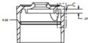
SECTION K-K SCALE 2 : 1
