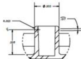
DETAIL L SCALE 4 : 1
